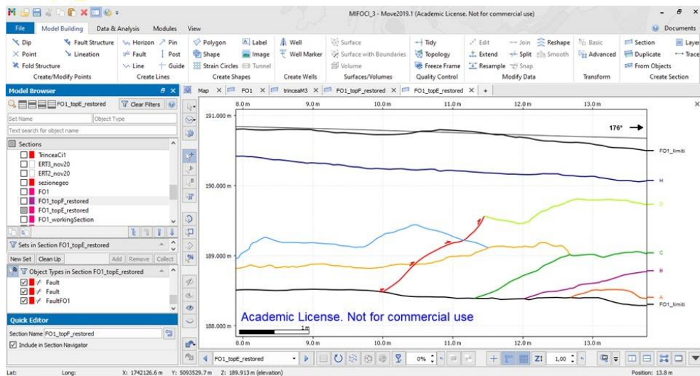
Fig.5. Follina1 trench restoration. Method: Fault Parallel Flow.
