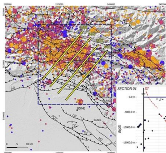
Fig.4. Seriated sections crossing the Susans-Tricesimo Thrust System (STTS), realized for the analysis of the hypocentral seismicity distribution with respect to the reconstructed faults geometry.
